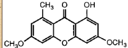
XANTHONE LICHEXANTHONE
